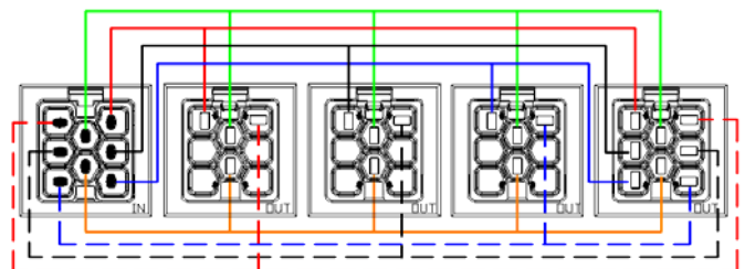
8-Wire 3L, 3N, 2G Phase Selector
