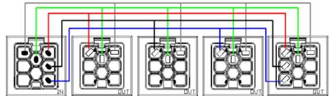
5-Wire 3-Phase Selector (347/600V 20A shown)
