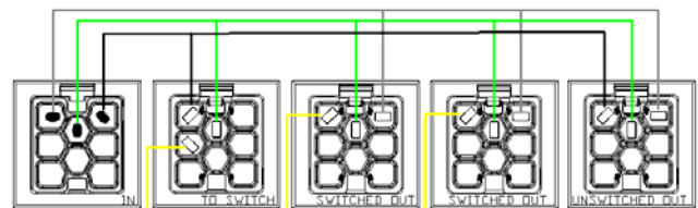
Single Circuit Switch Multi Tap (347/600V 20A shown)
