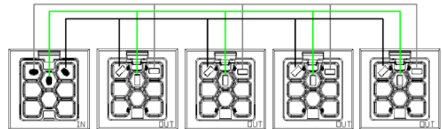
Single Circuit Multi Tap (347/600V 20A shown)
